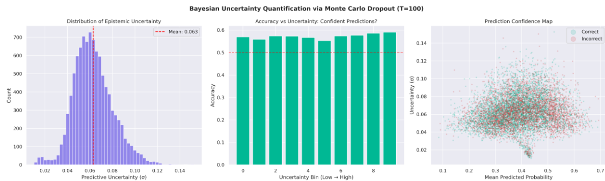
Figure 37: Monte Carlo Dropout Bayesian Epistemic Uncertainty Distribution
